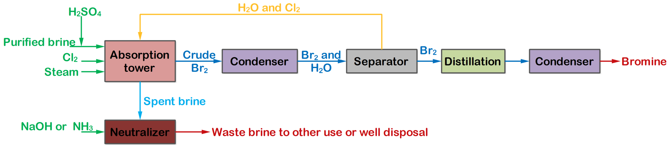
Figure: Manufacture of Bromine from sea water and brine
